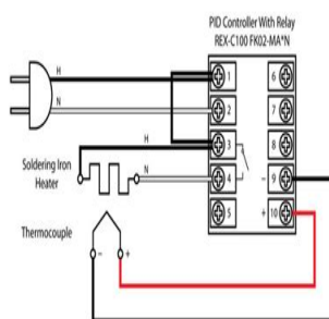
Soldering Iron PID Temperature Controller Wiring Diagram
